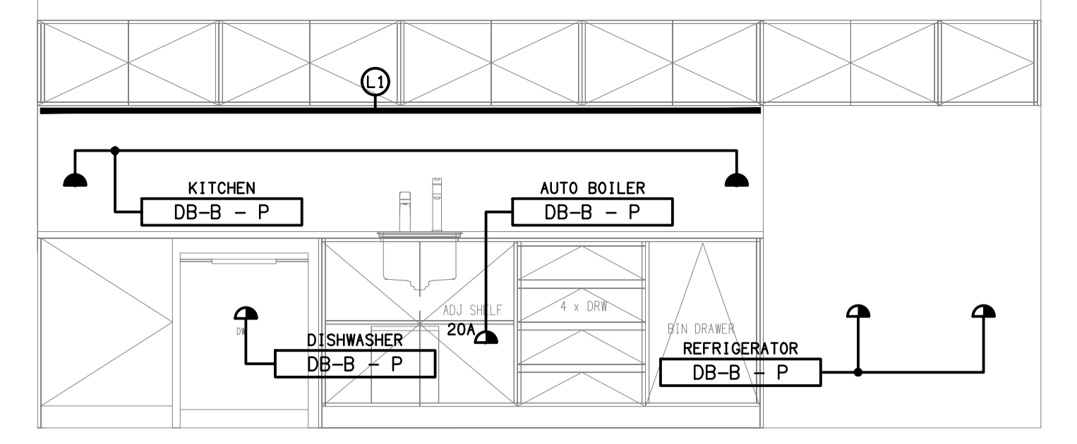
DETAIL A LUNCH ROOM 1 KITCHENETTE ELEVATION SCALE 1:25
