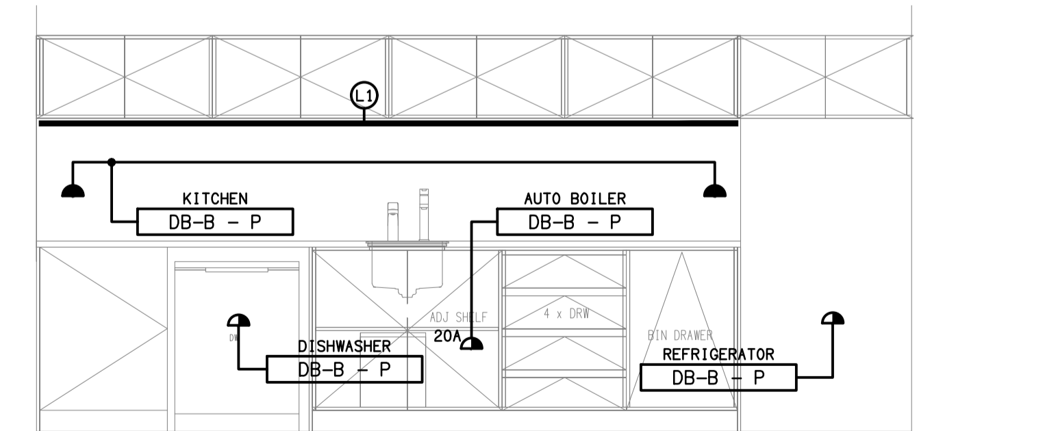
DETAIL D LUNCH ROOM 2 KITCHENETTE ELEVATION SCALE 1:25
