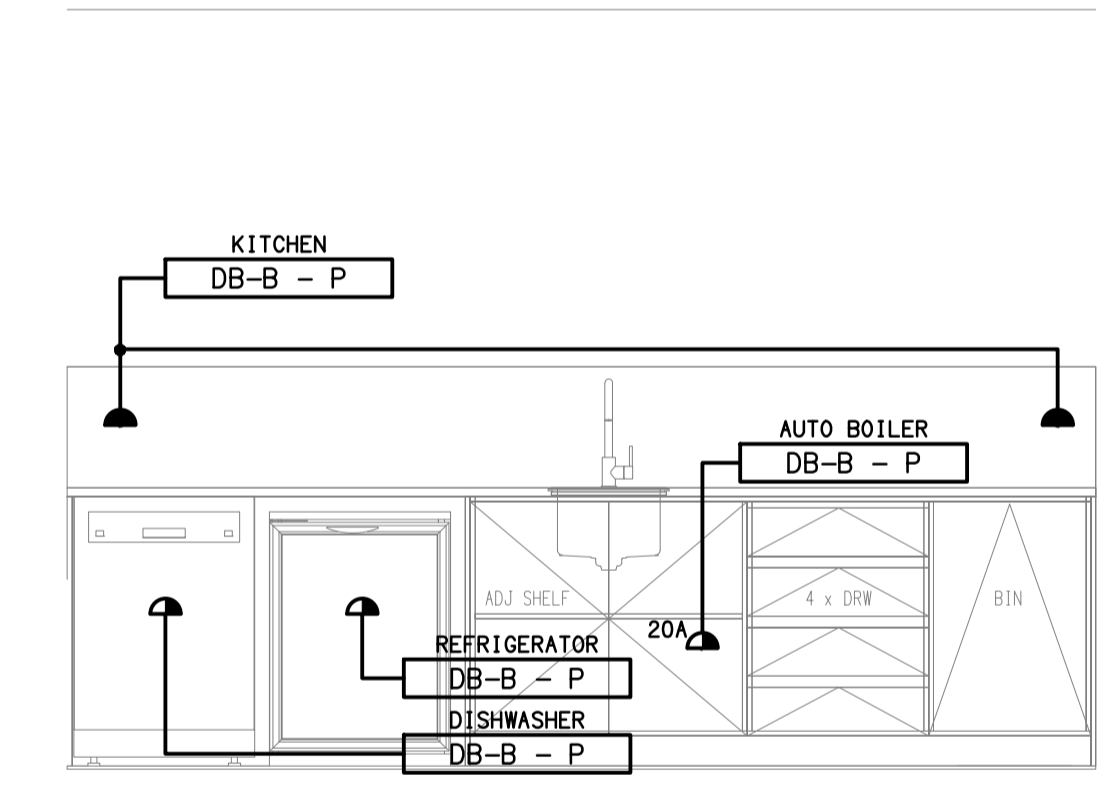
DETAIL C SHOWROOM CAFE KITCHENETTE SCALE 1:25
